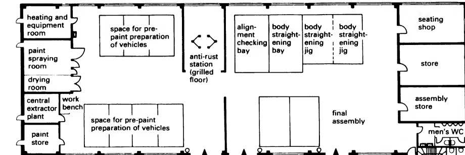
⑦ Example of plan for a repair shop (ground floor)
